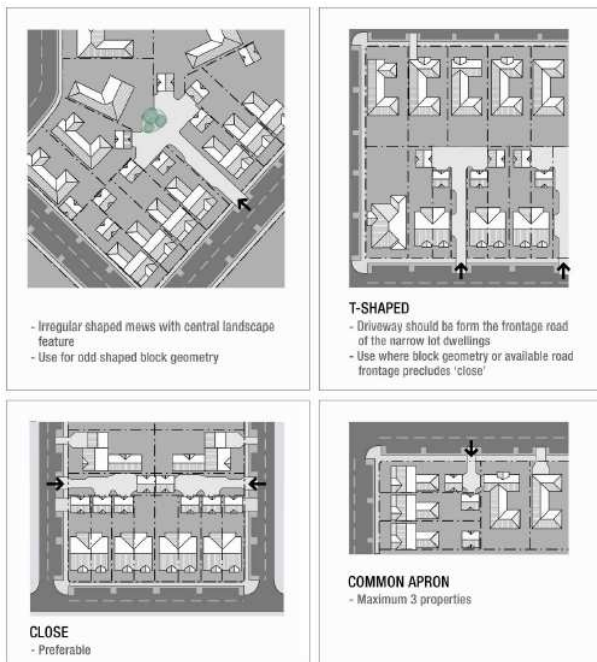
Figure 3-17: Indicative examples of shared driveways
