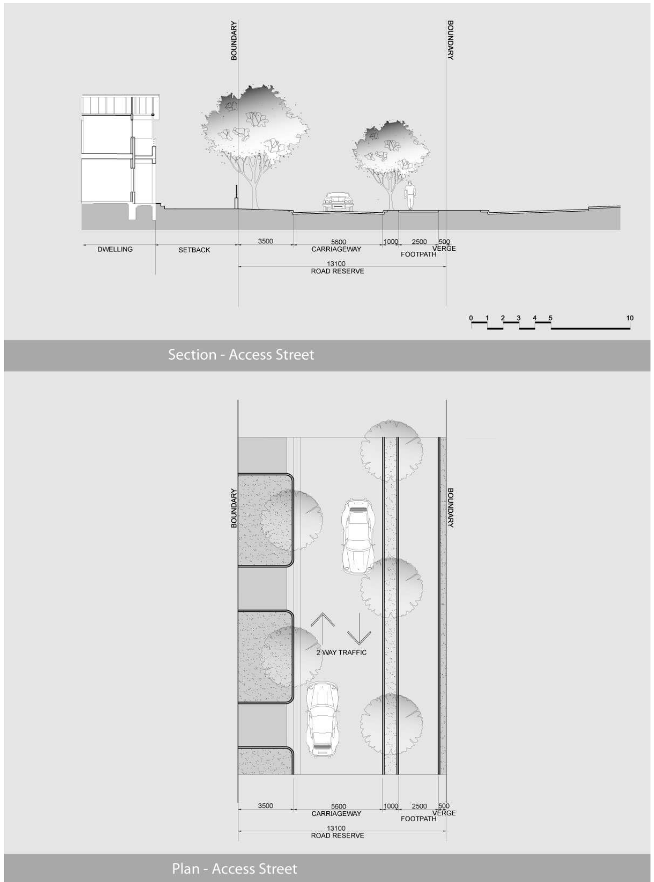
Figure 3-13: Typical access street
