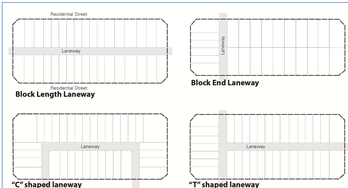
Figure 3-15: Sample lane layouts
