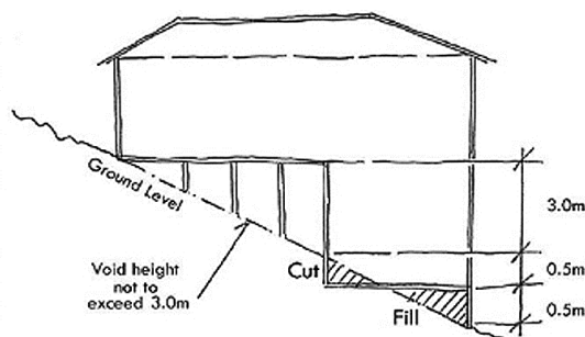
Figure 4-1: Maximum cut and fill within residential lots
